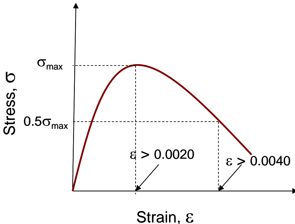
Figure S-1. Strain capacity requirements
